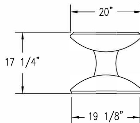
5 END VIEW Scale: 1/16" = 1"
