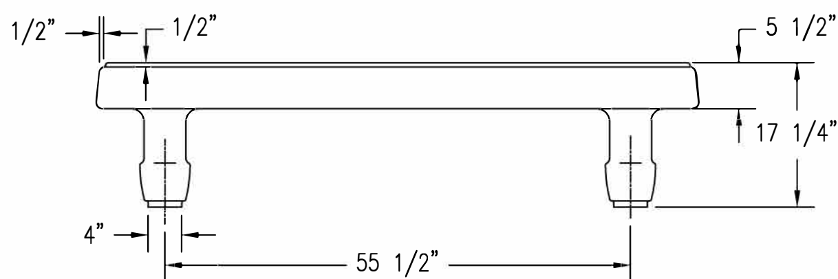
2 ELEVATION VIEW Scale: 1/16" = 1"
