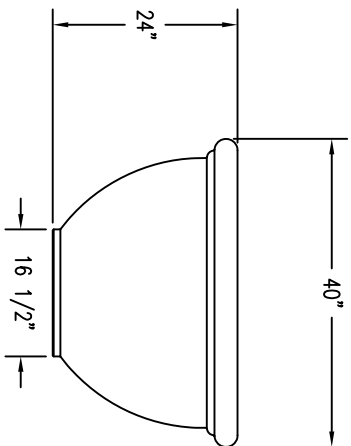
2 ELEVATION VIEW
