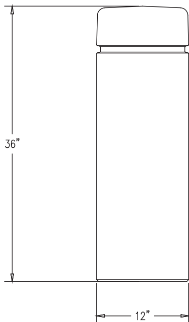
ELEVATION VIEW
