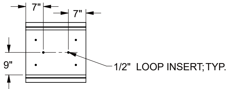
3 BOTTOM VIEW
