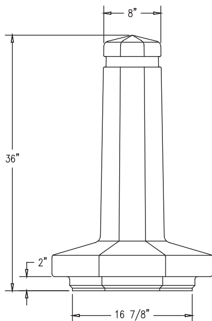
ELEVATION VIEW
