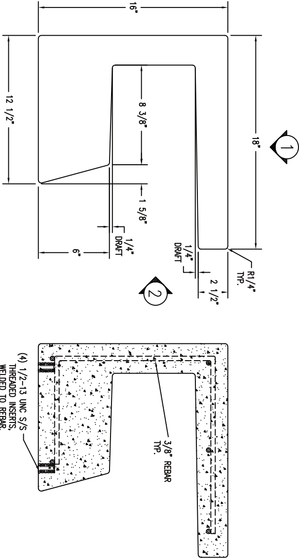
7 SECTION VIEW Scale: 1/4" = 1"
