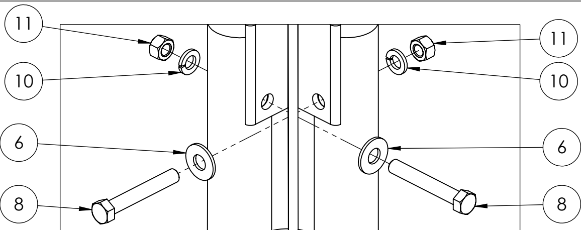
DETAIL B
