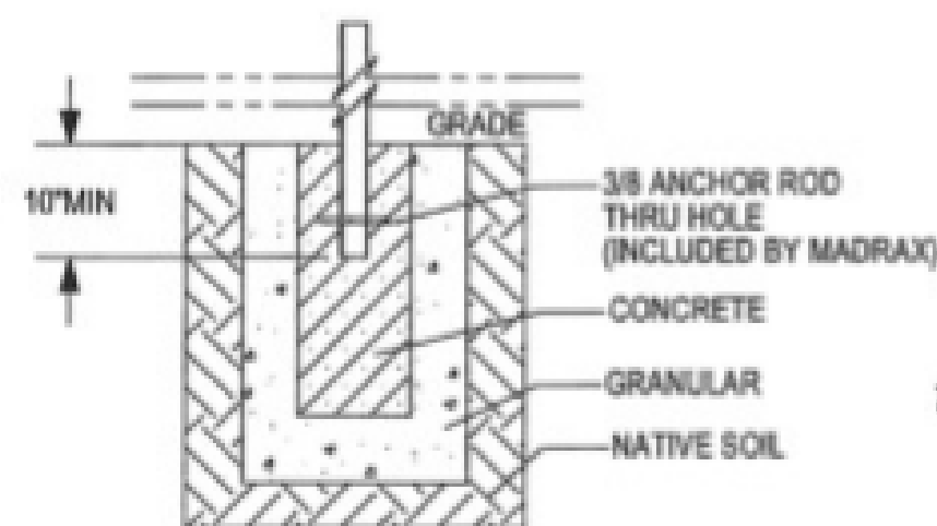
□ IN GROUND MOUNT (IG)
