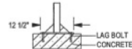
□ SURFACE GUSSET MOUNT (SG)
