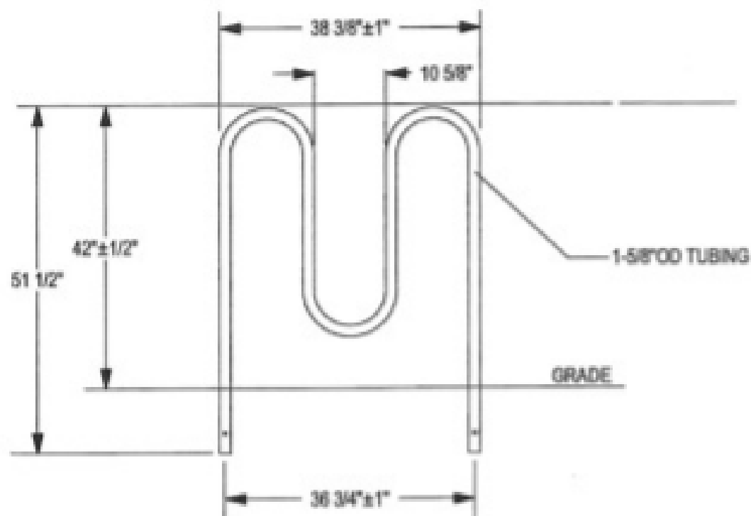
ELEVATION VIEW 3 LOOP - 5 BIKE CAPACITY
