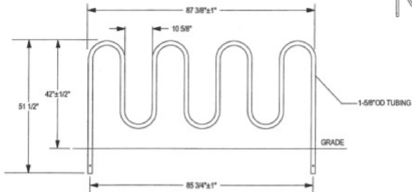
ELEVATION VIEW 7 LOOP - 9 BIKE CAPACITY
