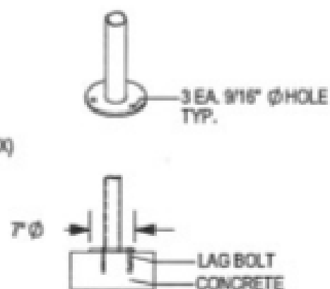
□ SURFACE FLANGE MOUNT (SF)
