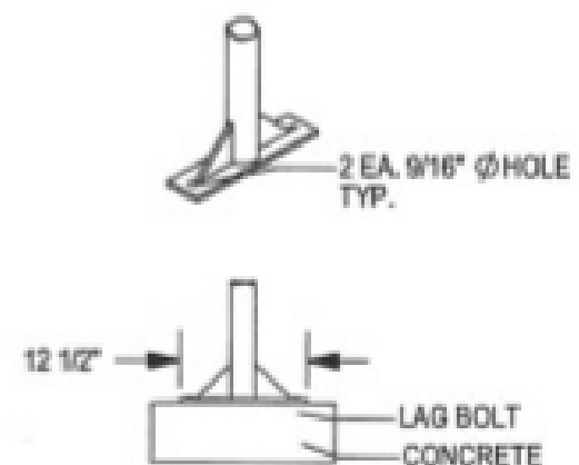
□ SURFACE GUSSET MOUNT (SG)
