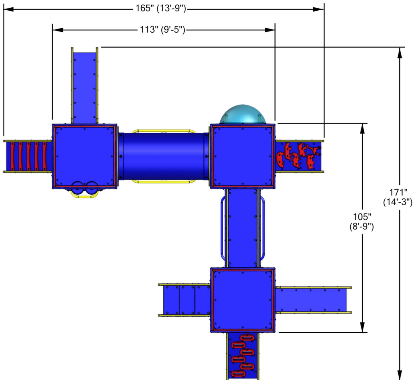
Plan View
