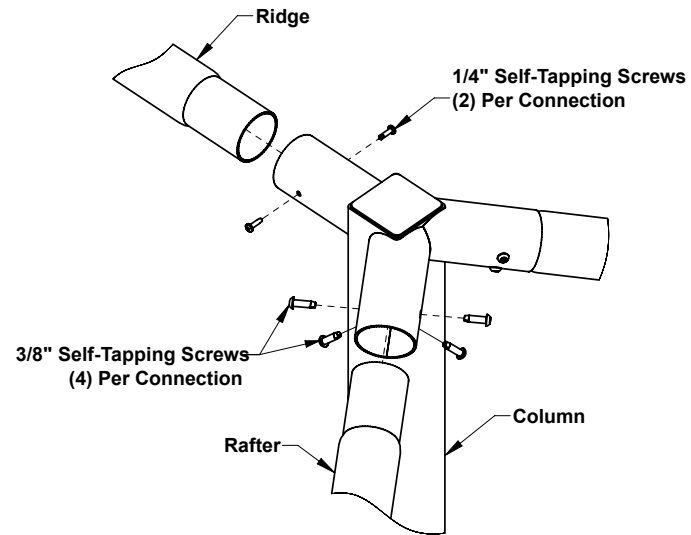
COLUMN-RIDGE-RAFTER CONNECTION
