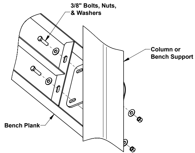
BENCH CONNECTION
